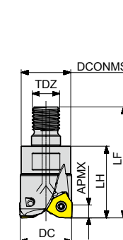
<M> Modular
