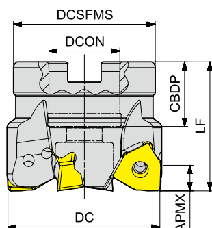
<S> Shellmill
